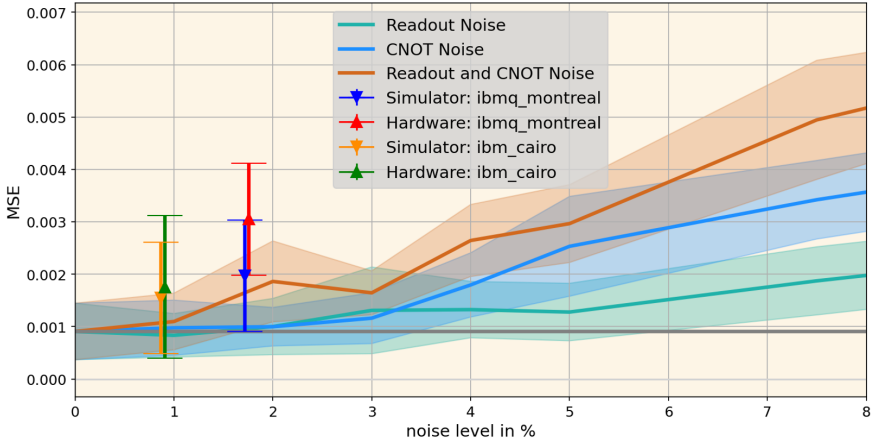
Fig. 10: Training noise study with various noise configurations, inclusive hardware noise simulations and training on the real hardware. The training with fake noise levels are repeated ten times.
