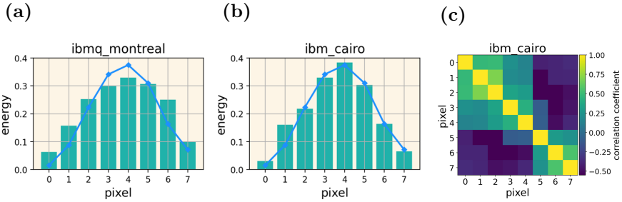
Fig. C3: On the left, the average shower images of the QAG model are trained on ibmq_montreal and in the middle on ibmq_cairo . The correlation plot on the right is created for the ibmq_cairo training.
