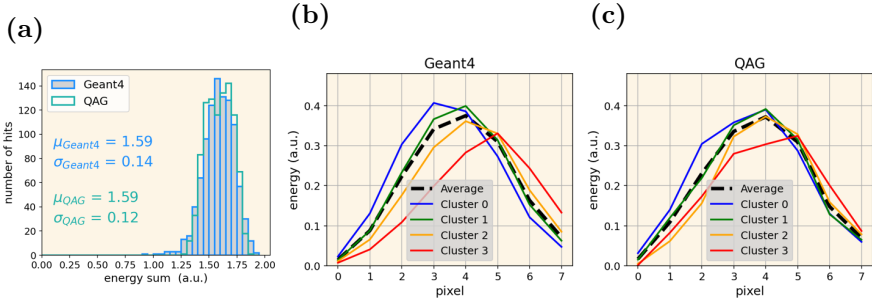
Fig. 7: (a) The energy sum histogram, (b) the four k-means clusters present in the images of Geant4, and (c) for QAG.
