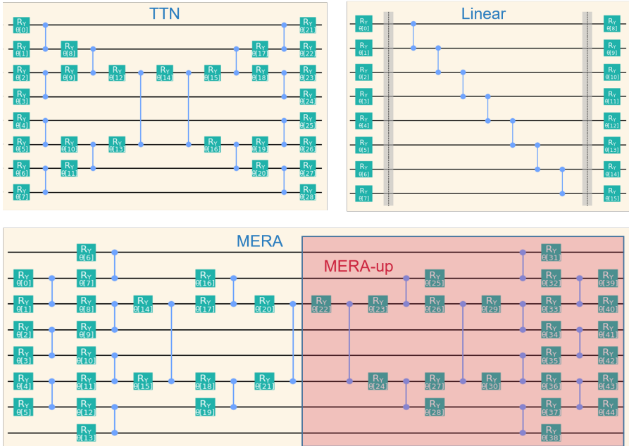
Fig. A1: The basic quantum circuit architectures under study. Top left: TTN architecture, top right: Linear entanglement architecture, bottom: the full circuit corresponds to the MERA architecture, with the red highlighted section corresponding to the MERA-up architecture.
