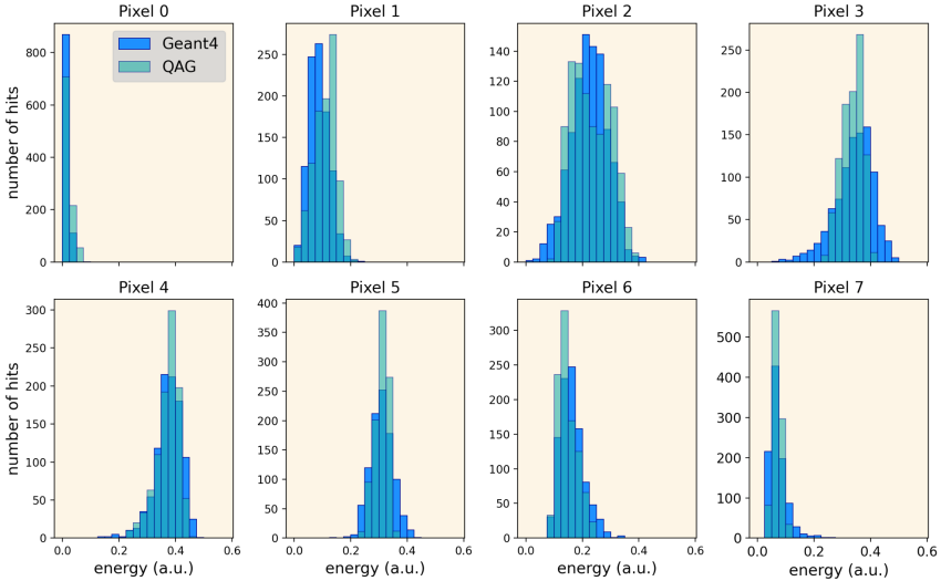
Fig. 8: Energy content histograms for the individual pixels for the Geant4 and the QAG model. The x-axis represents the energy depositions in one pixel and the y-axis the number of counts in each energy bin.
