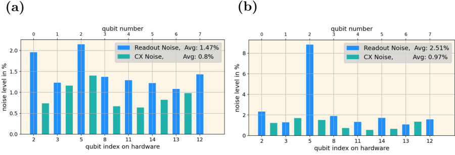
Fig. 11: The noise levels of the ibmq_montreal device are shown on the left before and on the right after the calibration change during training. The inference tests are performed with the right noise model. It can be seen, that the readout noise of qubit number five increased from two to over eight percent.
