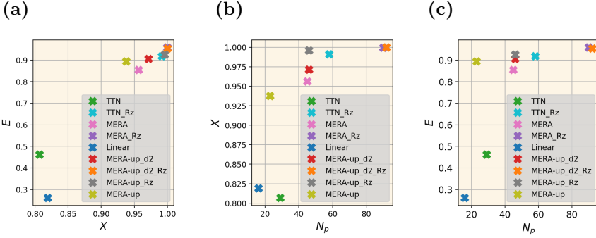
Fig. B2: Study of potential correlations between the three characteristic circuit numbers. On the left: X versus E . In the middle: N_p versus X . On the right: N_p versus E .
