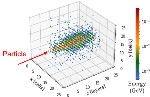
Fig. 1: An example 3D calorimeter shower image.
