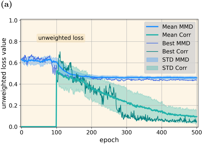
Fig. 5: The unweighted loss values as a function of the training epochs.
